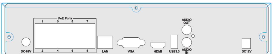
Fig 2-2 Rear Panel for 16-ch
