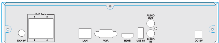
Fig 2-1 Rear Panel for 8-ch
